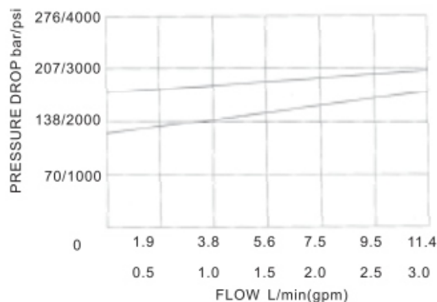
Pressure drop-flow curve 32 cST Oil/45°C
