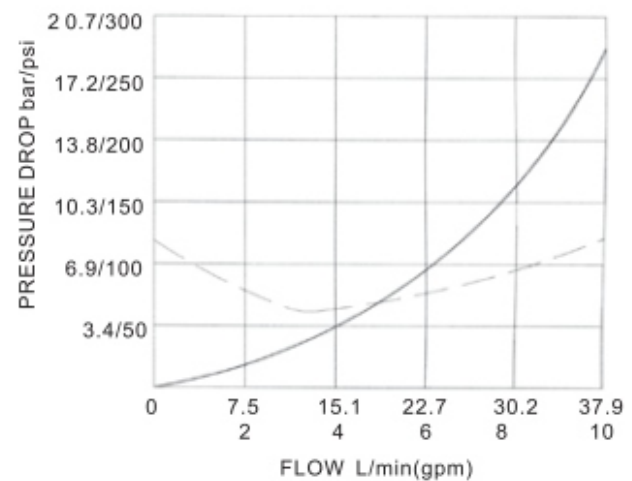
Pressure drop-flow curve 32 cST Oil/45°C P—T ——— T—P - - -
